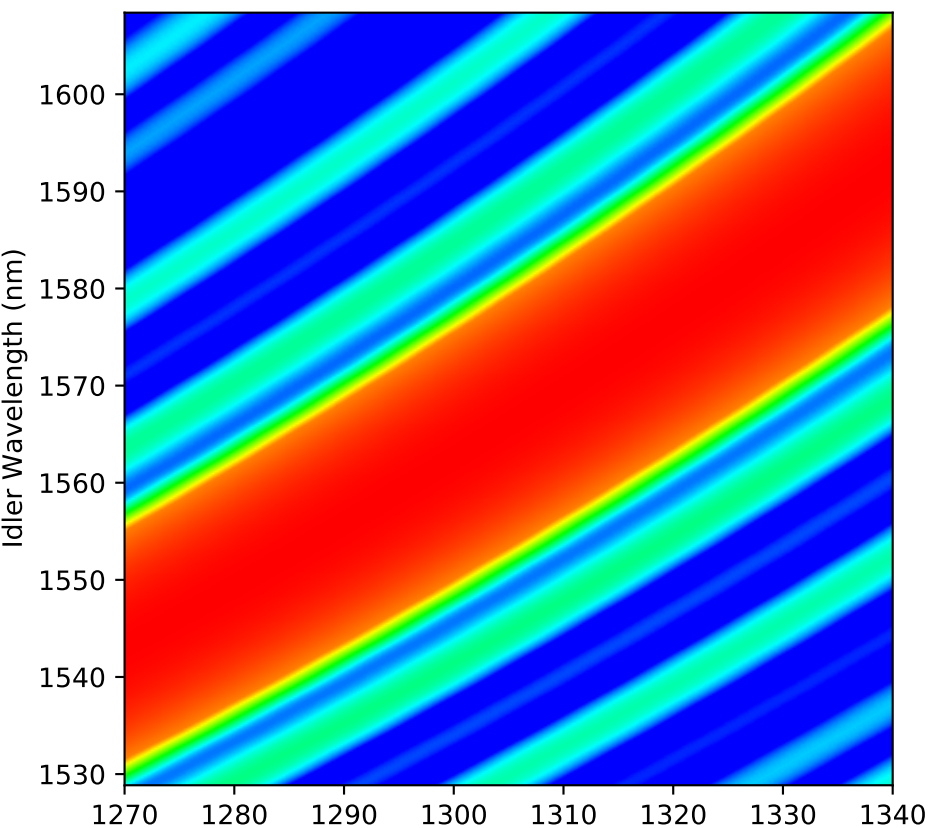
3. Optimized JSA (Theory, Log) Pump=3.09nm | purity=0.9963
