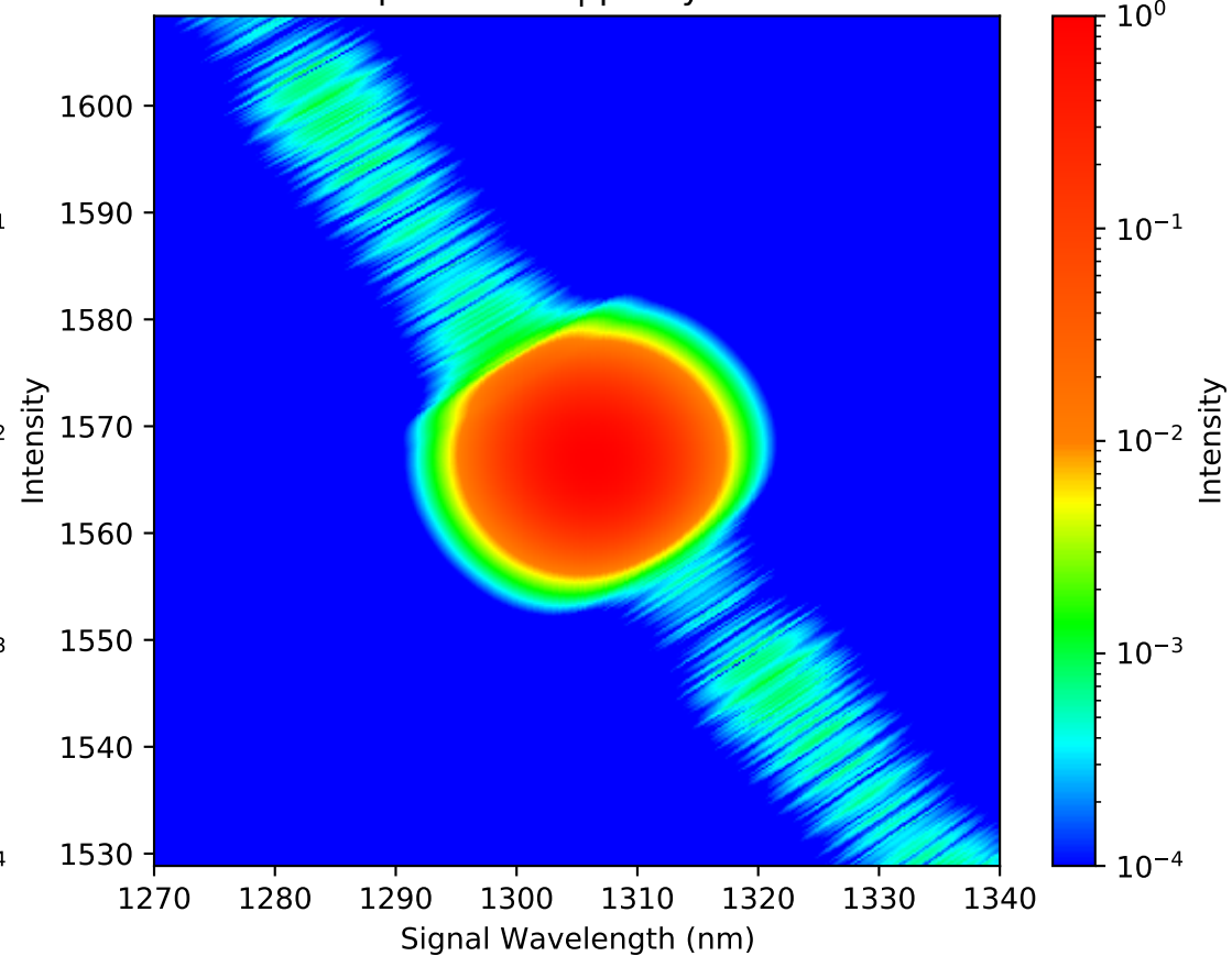
4. Optimized JSA (Exp Reconstruction, Log) Pump=3.08nm | purity=0.9925
