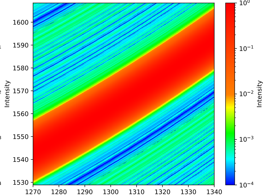
4. Optimized JSA (Exp Reconstruction, Log) Pump=3.08nm | purity=0.9925
