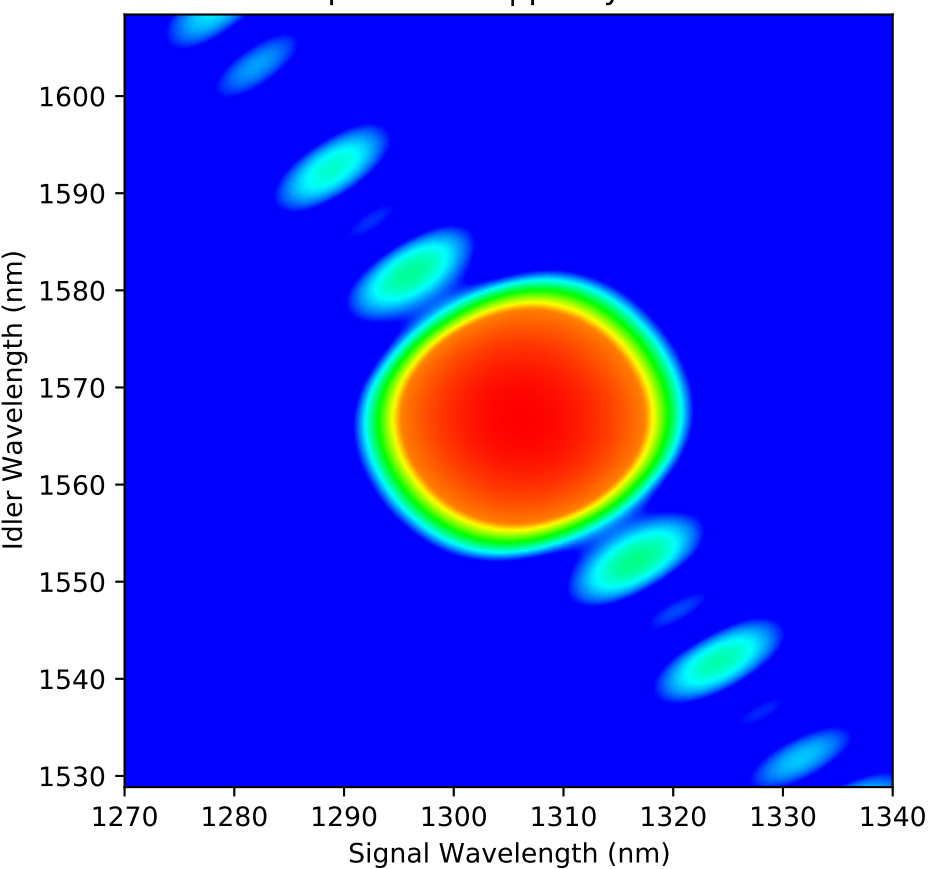
3. Optimized JSA (Theory, Log) Pump=3.09nm | purity=0.9963
